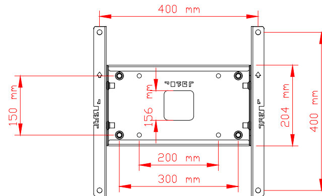
PLW Bracket
