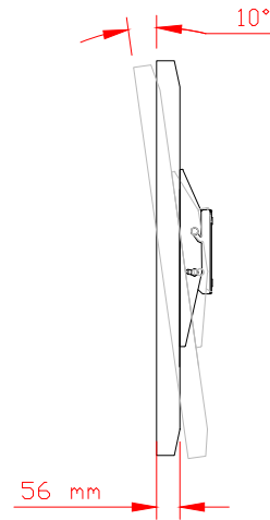
PLW Bracket
