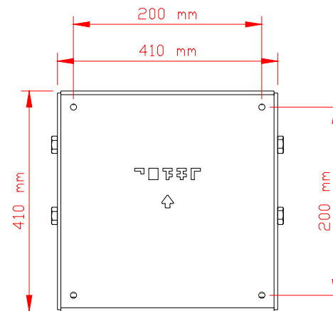
Unicol PLW Bracket
