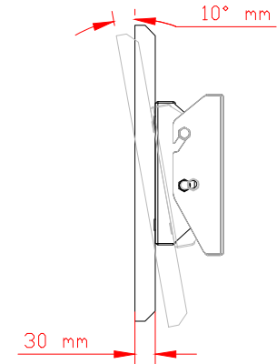
Rear View with PLW Bracket
