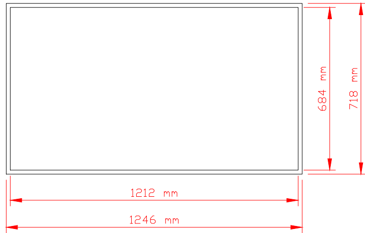
Rear View With PLW Bracket
