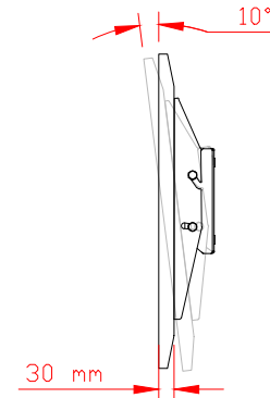
Side View with PLW Bracket
